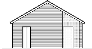
Proposed East Elevation
